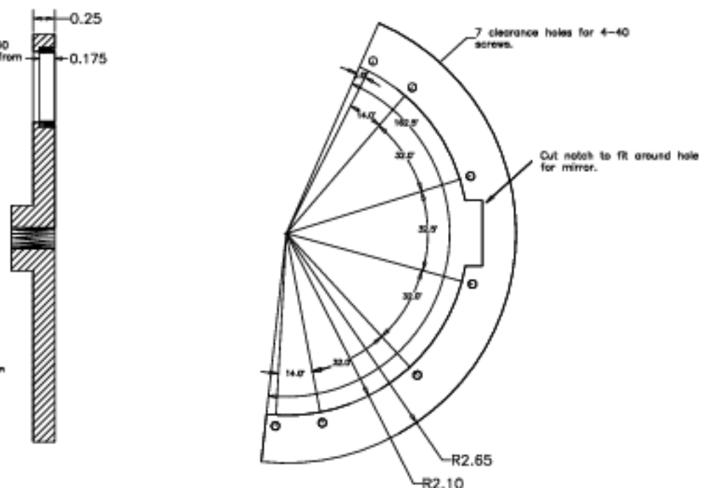
Part 28-015, Circular Mask for Limit Switches. Make of aluminum sheet metal. (1 reqd)
