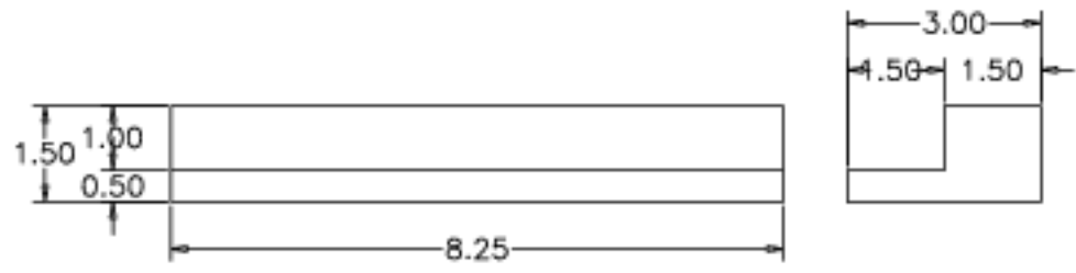
Cradle for CCD Dewar (part is 11 inches deep)
