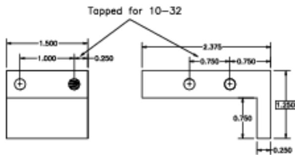
Part 24-034, Grating Retainer. Make of aluminum. (1 reqd)
