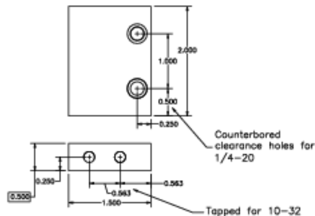
Part 24-023, Standoff. Make of 1/2-inch aluminum plate. (1 reqd)
