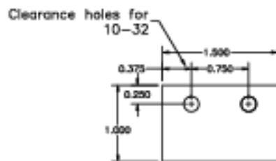
Part 24-036, Clip (lateral grating retainer). Make of 1/8-inch aluminum strap. (1 reqd)
