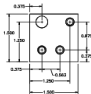
Part 24-029, Positioning clip, no. 2. Make of 3/8-inch aluminum plate. (1 reqd)
