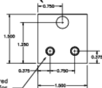
Part 24-028, Positioning clip, no. 1. Make of 3/8-inch aluminum plate. (1 reqd)
