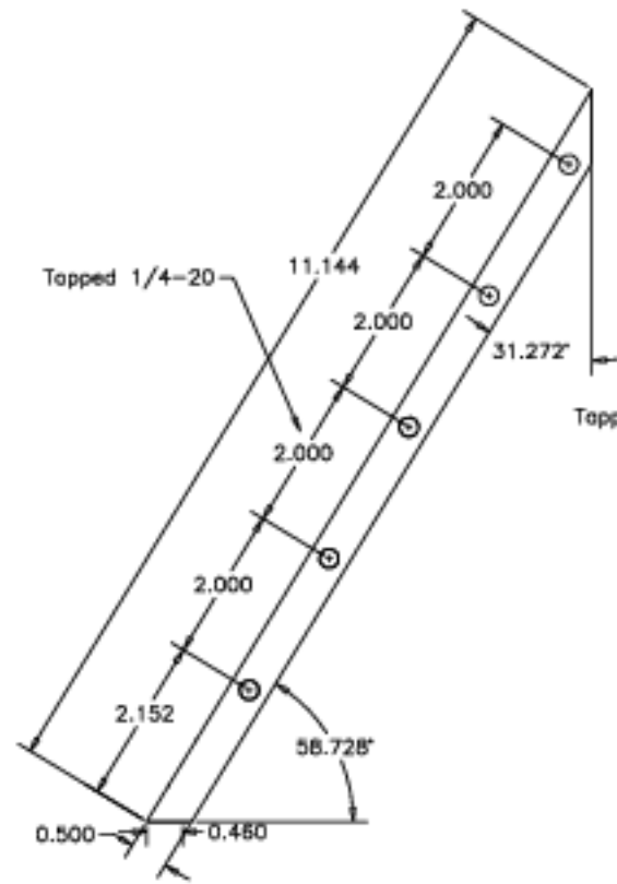
Part 24-024, Back stiffener for grating stand. Make of 1/2-inch aluminum plate. (1 reqd)
