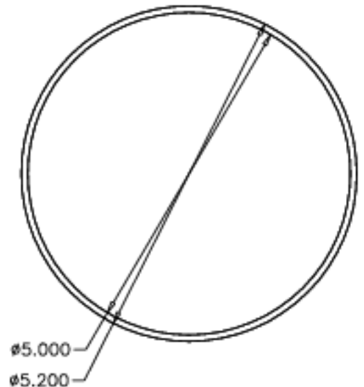
Part 24-015, Bearing spacer. Make of aluminum. (1 reqd)
