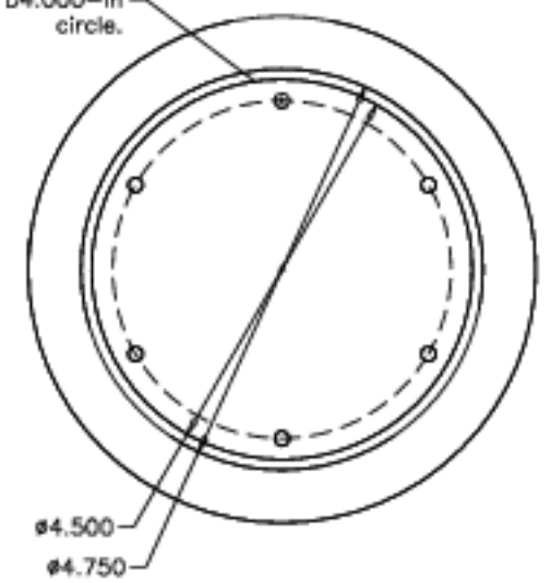
Bottom View of Part
