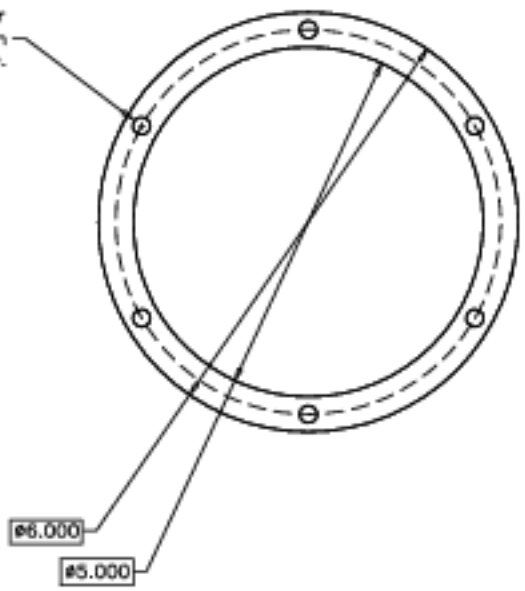
Bottom View of Part
