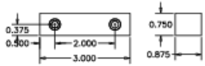
Part 23-030, Grating Stop, Type 2. Make out of aluminum. (2 reqd)
