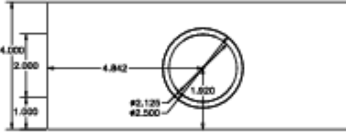
Part 23-018, Back Lateral Frame (upper). Make out of 3/4-inch aluminum plate (1 reqd)
