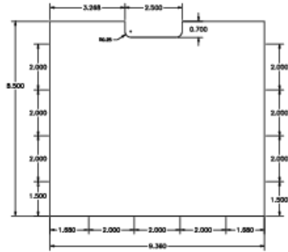
Part 23-017, Back Lateral Frame (lower). Make out of 0.5-inch aluminum plate (1 reqd)
