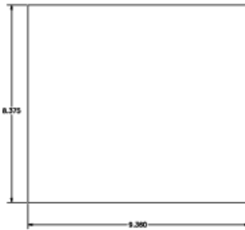
Part 23-014, Interior Lateral Frame (gusset). Make out of 0.5-inch aluminum plate. Get hole pattern for edges from 23-015. (1 reqd)
