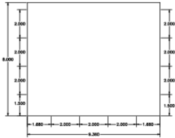
Part 23-015, Front Lateral Frame (lower). Make out of 0.5-inch aluminum plate (1 reqd)
