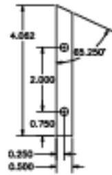
Part 23-018, Back Lateral Frame (upper). Make out of 3/4-inch aluminum plate (1 reqd)
