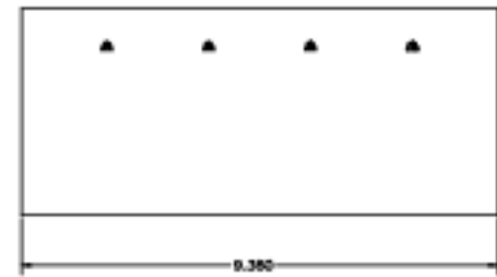
Part 23-016, Front Lateral Frame (upper). Make out of 0.5-inch aluminum plate (1 reqd)
