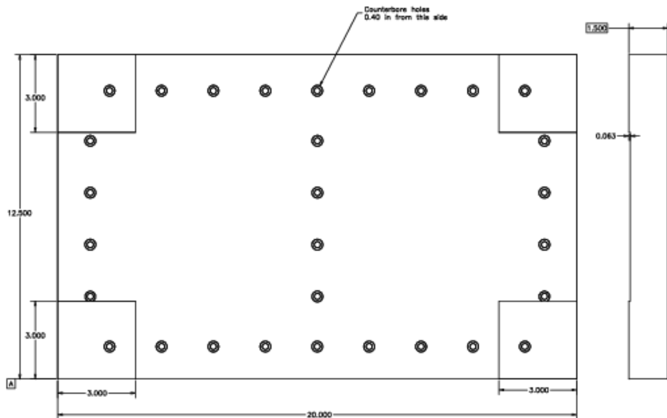
Bottom View of Part
