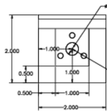
Part 22-003a, Horizontal Puck for supporting mirror. Make of invar. (4 reqd)
