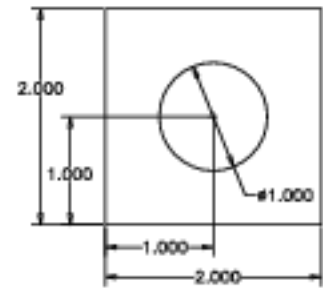
Part 22-004, Vertical Puck for supporting mirror. Make of invar. (2 reqd)
