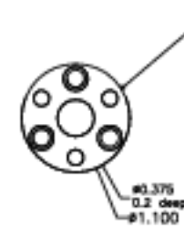
3 holes tapped 8-32, alternated with 3 counterbored holes for 8-32, on R0.400 circle
