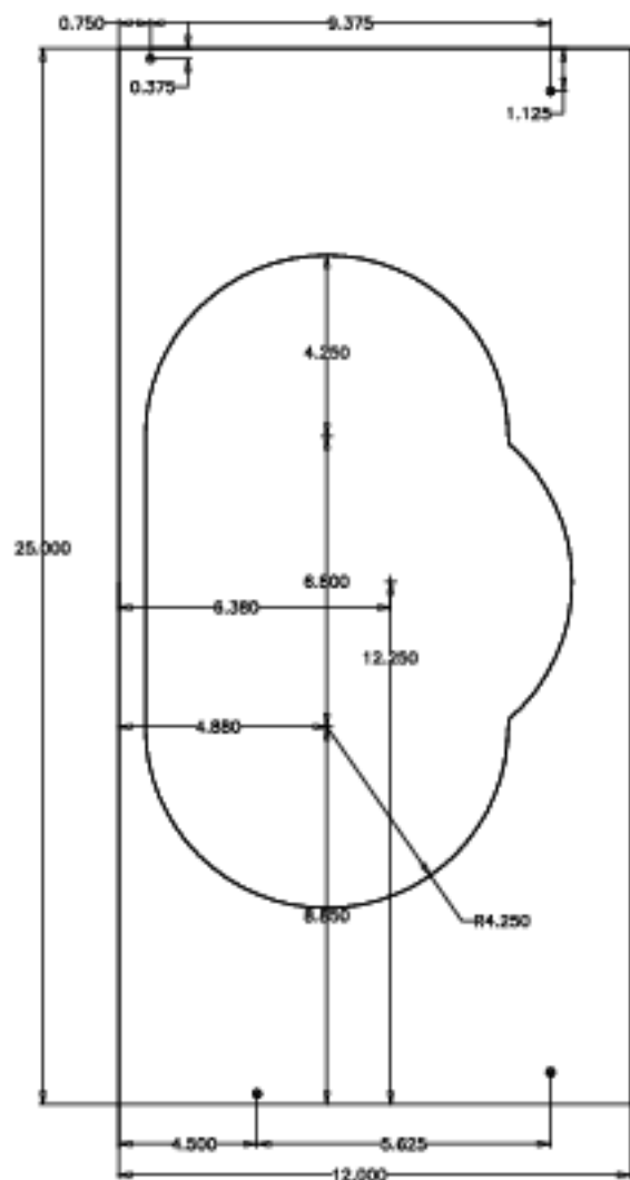
Part 22-019, Baffle for Collimator. Make of 0.05-in aluminum sheet. (1 reqd)
