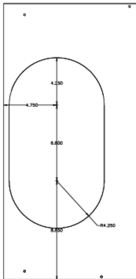
Part 22-020, Baffle for Second, Reimaging Mirror. Make of 0.05-in aluminum sheet. (1 reqd)
