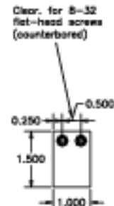
Part 22-016, Mirror retaining clip. Make of 1/8x1-in aluminum strap. (6 reqd)
