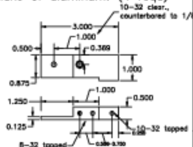
Part 22-018, Standoff (mirror retainer), type 2. Make of aluminum. (2 reqd, one a MIRROR IMAGE of the part shown)
