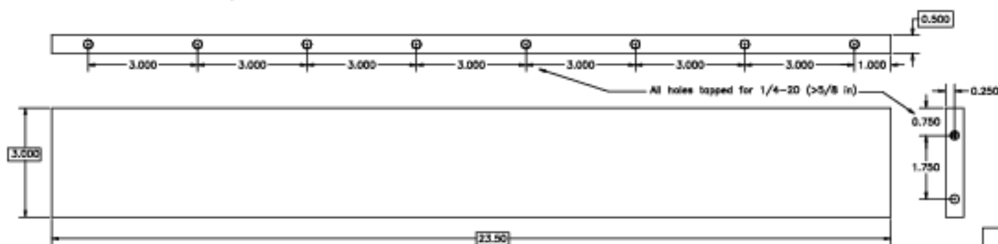
Part 22-013, Vertical Gusset for Collimator Stand. Make of 0.5-in aluminum plate. (B reqd)
