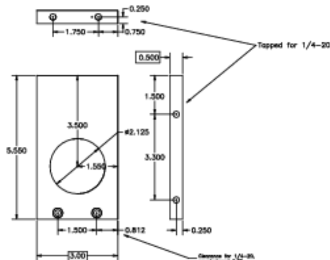
Part 22-014, Lateral-Support Frame for Collimator Stand, 1. Make of 0.5x3-in aluminum strap. (4 reqd; 2 of which are MIRROR IMAGES of the one shown here)
