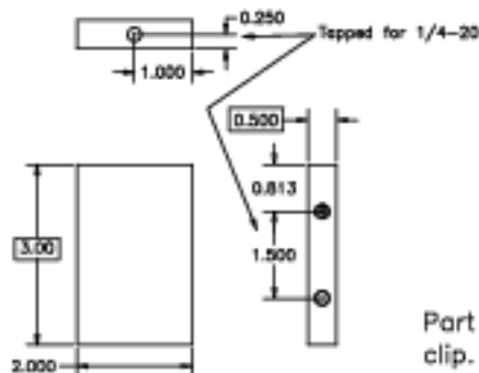
Part 22-015, Lateral-Support Frame for Collimator Stand, 2. Make of 0.5x3-in aluminum strap. (4 reqd)
