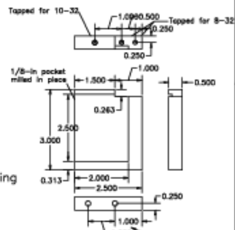
Part 22-017, Standoff (mirror retainer), type 1. Make of aluminum. (4 reqd)
