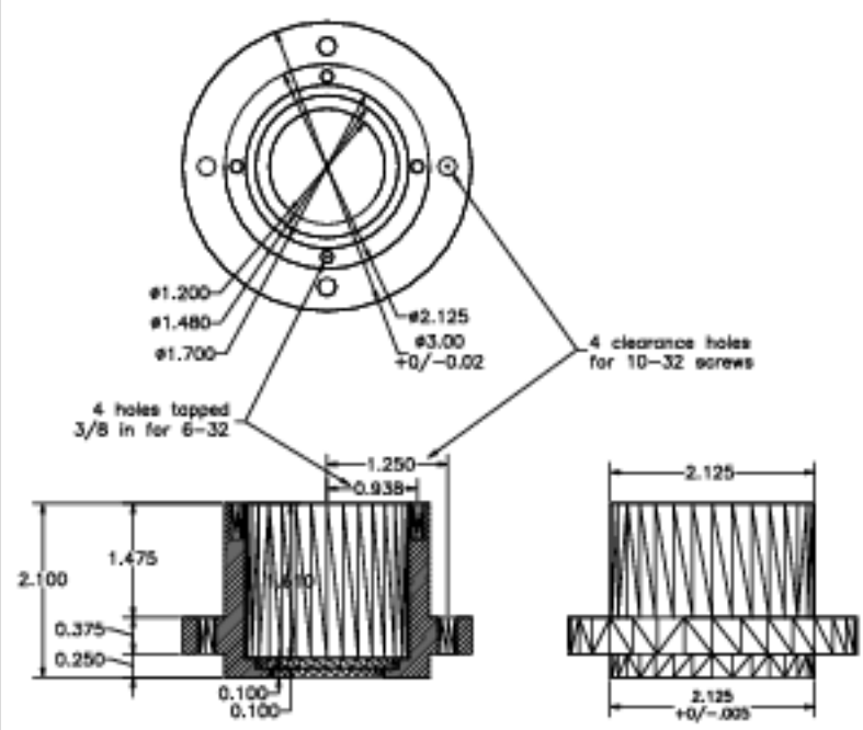
Part 22-031, Locator Body. Aluminum rod. Make 20.
