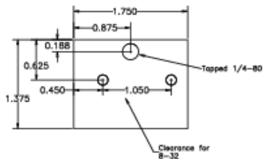
part 21-033, Back Mirror Retainer. Aluminum, 0.25 thick (2 reqd)
