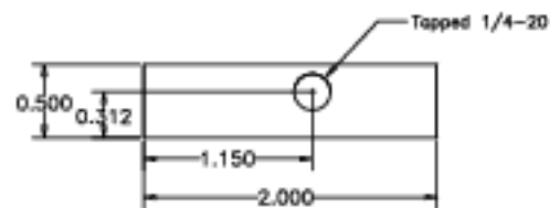
Part 21-034, Bottom Inside Mirror Retainer. Aluminum. (1 reqd)
