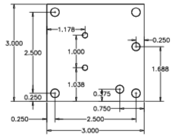
Part 21-042, Base for Low-Dispersion Feed. 1/4-inch aluminum plate. (1 reqd)
