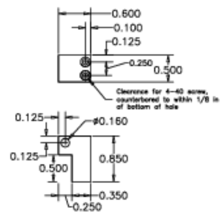
Part 21-012/49, Holder for Limit Switch, Back. Aluminum (2 reqd, one for each slide)
