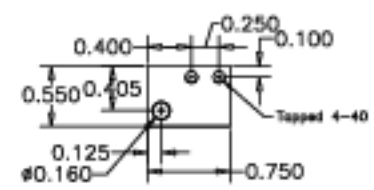
Part 21-011/48, Holder for Limit Switch, Front. 3/8-in aluminum plate. (2 reqd, one for each slide)
