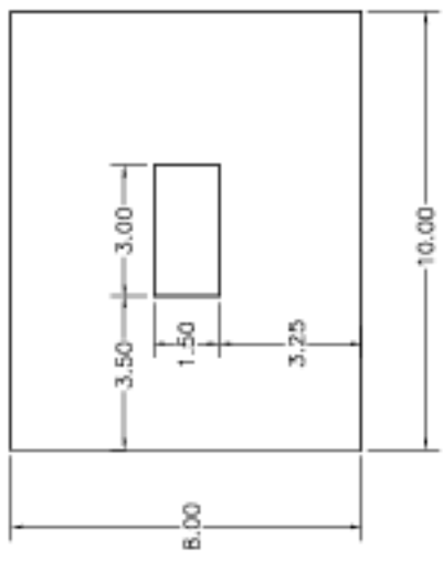
Part 20-051, Top (Base) Plate. Make of 7/8-in steel plate (1 reqd/carriage, 10 total)
