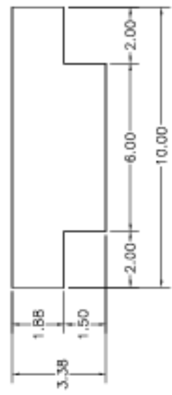
Part 20-052, Side Plate. Make of 1-in steel plate. (2 reqd/carriage, 20 in all)
