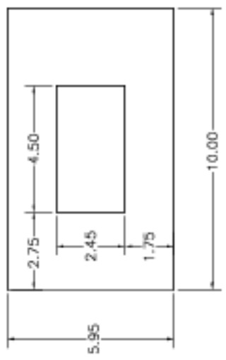
Part 20-054, Bottom Plate. Make of 3/4-in steel plate. (1 reqd/carriage, 10 in all)
