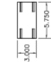
Part 10-024, Top Stiffener of Altitude Drive Attachment. Make of 1-in aluminum plate. Holes in the two ends (one shown for illustration) are 1.5 in deep and tapped for 3/8-16 screws (1 reqd)
