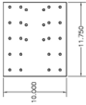
Part 10-020, Base Plate of Altitude Drive Attachment. Make of 1-in aluminum plate. (1 reqd)
