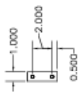
Part 10-024, Top Stiffener of Altitude Drive Attachment. Make of 1-in aluminum plate. Holes in the two ends (one shown for illustration) are 1.5 in deep and tapped for 3/8-16 screws (1 reqd)
