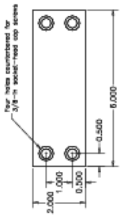
Part 7-122, Cross Piece. 1/2-in aluminum plate. One reqd.
