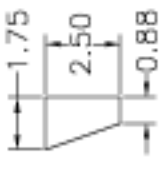
Part 5-053, External Stiffener. Make of 1/8-inch stainless steel plate. (8 reqd)
