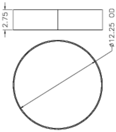
Part 5-051, Wall Cylinder of Instrument Head. Make of 1/8-inch stainless steel plate. (1 reqd)
