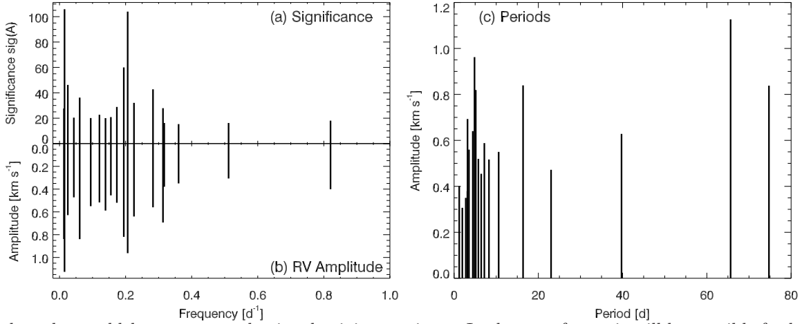
FIG. 3.— Left: Detected frequencies with their corresponding significance level (panel a) and radial velocity amplitude (panel b). Given the weak magnetic field on Rigel, rotational modulations induced by stellar spots are unlikely. Right: Perioda distribution of detected modes with their corresponding amplitude.
