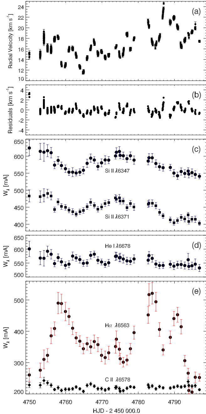
FIG. 2.— (a) A representative 50 day radial velocity curve of Rigel. 1- \sigma error in RV is overplotted. (b) A residual plot with 19 harmonics removed as in Table 2 with rms deviation 0.59 km s -1 . (c) The 1-day binned EW measures of two metallic lines, namely Si II \lambda 6347 and Si II \lambda 6371 Å which exhibit significant temporal variations. (d) A similar plot for the He I \lambda 6678 line, and (e) for C II \lambda 6578 and H \alpha lines.
