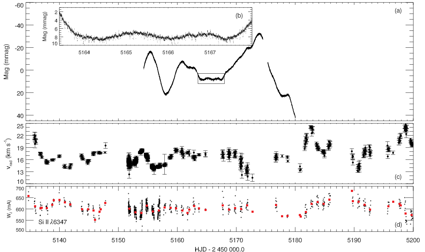
FIG. 1.— Compilation of observations from the Rigel campaign. Panel (a) shows the 27.7-day MOST space photometry (Section 3.1). Panel (b) is a 5-day zoomed-in portion of the data to emphasize the amplitude and time scale of the shortest variations. Panel (c) shows the RV data which demonstrates a correlation with the flux changes (Section 3.2). Panel (d) is the equivalent width variation for Si II \lambda 6347.1 Å during the same monitoring epoch (Section 3.4); the (red) squares are the 1-day binned averages (see Figure 2).
